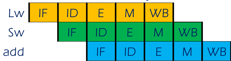
Pipeline: 7 cycles, cycles time = 1 secs
