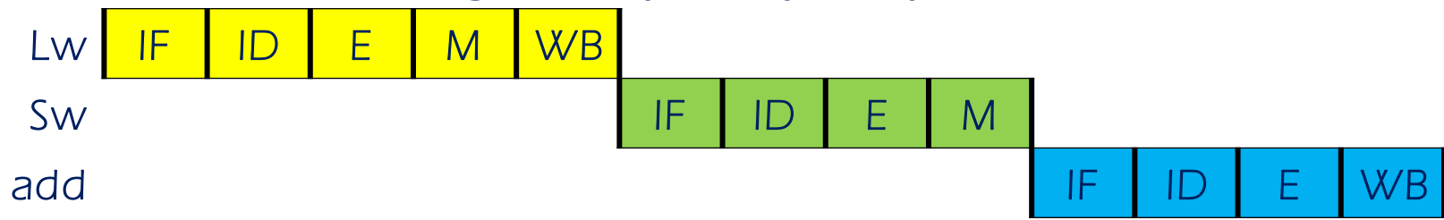
Multi clock cycle: 5 + 4 + 4 = 13 cycles, cycle time = 1 secs
